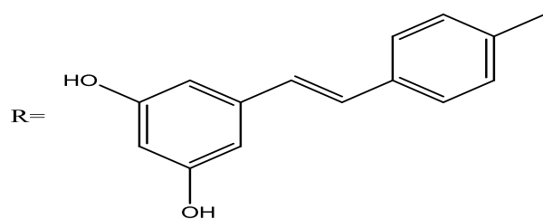
Scheme 6. Mechanism of 3,5,4'-tri-O-isobutyryl synthesis resveratrol using esterification of reseveratrol
