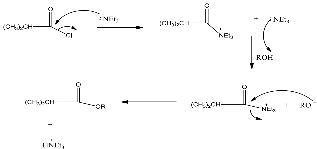
Scheme 5. Synthesis of 3,5,4'-tri-O-isobutyryl resveratrol ( Esterification)
