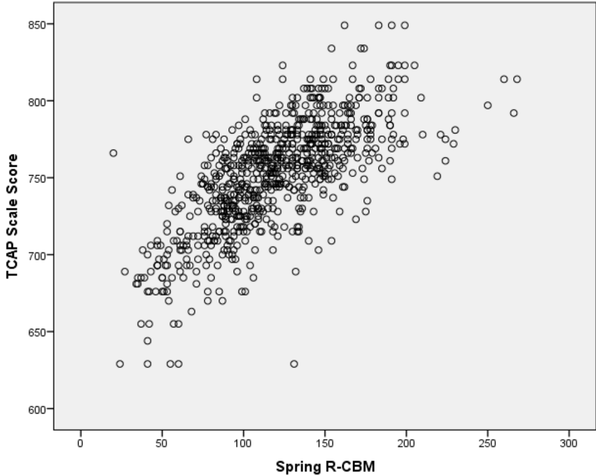
Figure 3. Scatterplot Depicting the Relationship Between Standardized Spring R-CBM Scores and TCAP Reading Scores.
