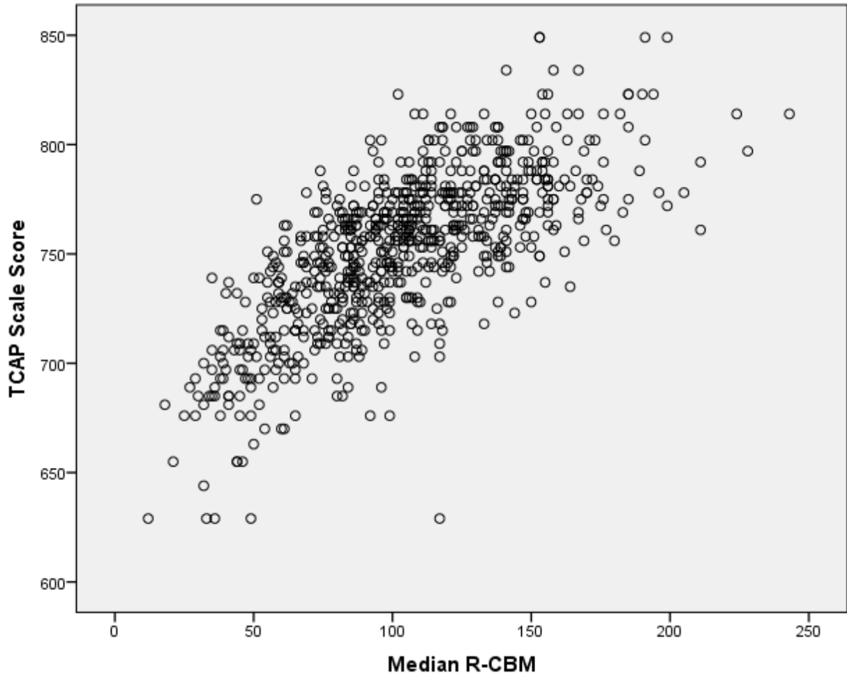
Figure 3. Scatterplot Depicting the Relationship Between Standardized Median R-CBM Scores and TCAP Reading Scores.
