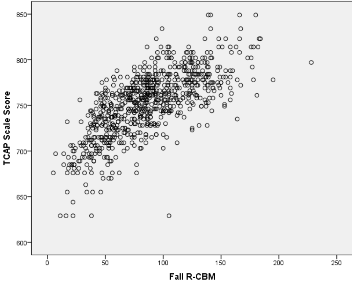
Figure 1. Scatterplot Depicting the Relationship Between Standardized Fall R-CBM Scores and TCAP Reading Scores.
