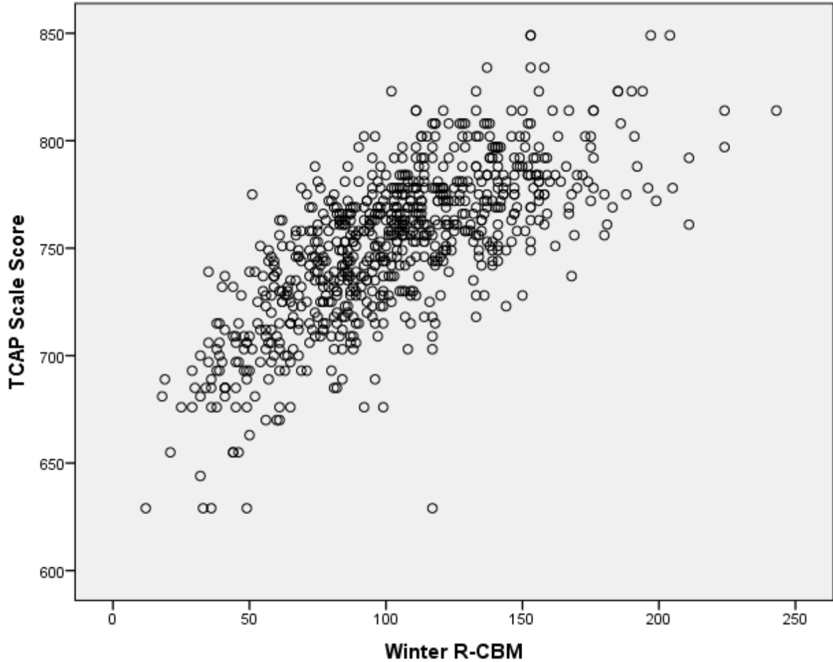
Figure 2. Scatterplot Depicting the Relationship Between Standardized Winter R-CBM Scores and TCAP Reading Scores.
