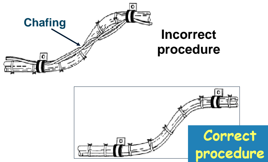
Figure 10. Adding or Replacing Wires on a Bundle (Aircraft Wiring Practices, 2002).
