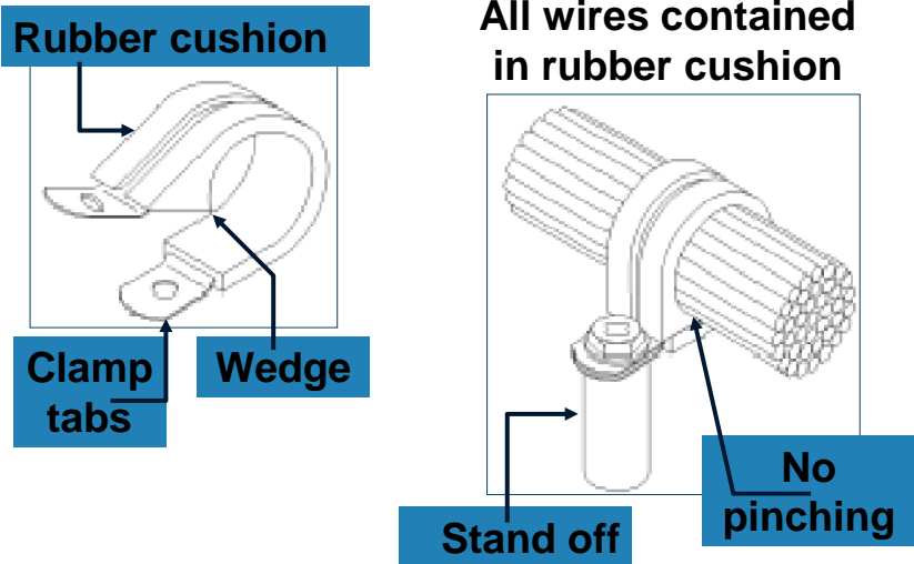
Figure 5. Typical Rubber Clamp (Aircraft Wiring Practices, 2002).
