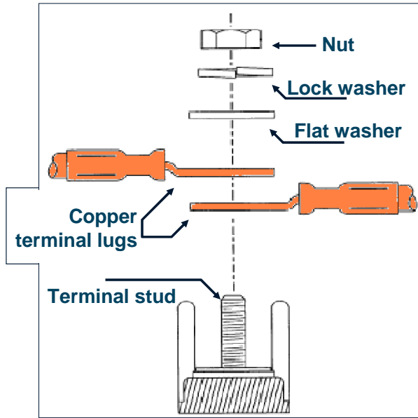
Figure 12. Terminal Stacking Like Materials (Aircraft Wiring Practices, 2002).
