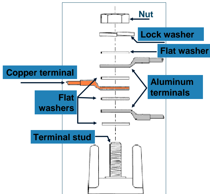
Figure 13. Terminal Stacking Unlike Materials (Aircraft Wiring Practices, 2002).
