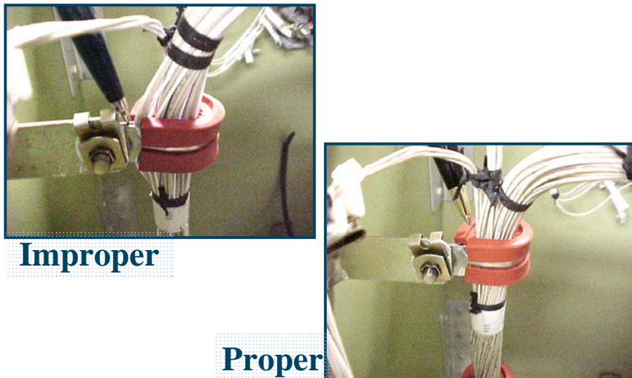
Figure 6. Clamping (Aircraft Wiring Practices, 2002).
