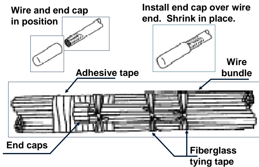
Figure 8. Spare Wire Termination Using Endcap (Aircraft Wiring Practices, 2002).
