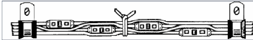
Figure 11. Staggered Splices (Aircraft Wiring Practices, 2002).
