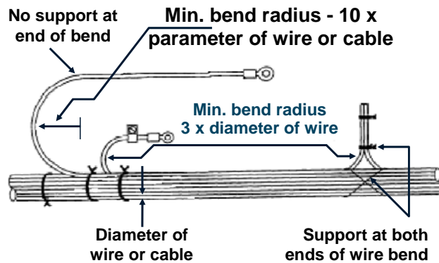
Figure 7. Minimum Bend Radii (Aircraft Wiring Practices, 2002).
