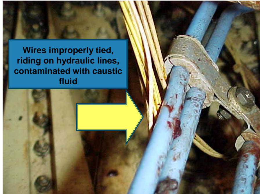
Figure 4. Wires Improperly Routed (Aircraft Wiring Practices, 2002).
