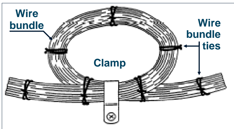
Coil and stow short/long wire bundles in low vibration areas
