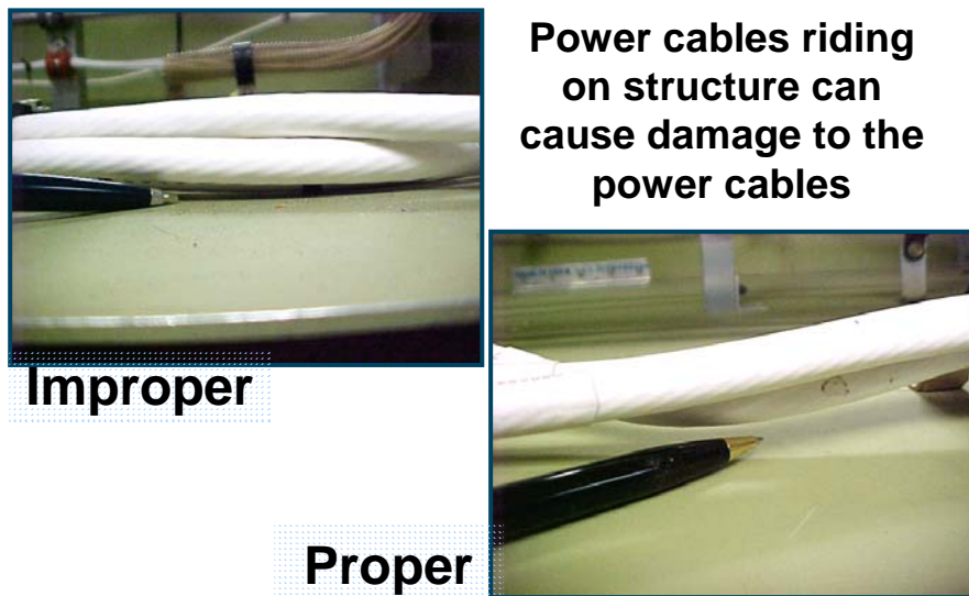
Figure 3. Wires Riding On Structure (Aircraft Wiring Practices, 2002).
