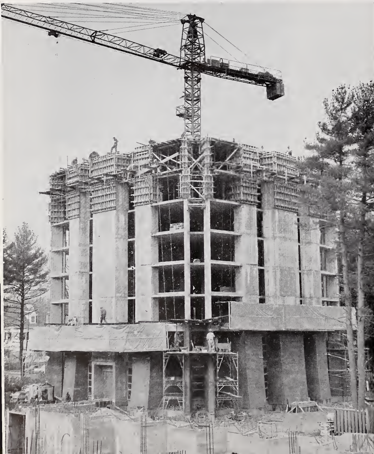
Shown here is the residential tower of the Senior Center after nine of the sixteen floors had been laid. The red brick design so familiar to Bowdoin men can be seen at the foot of the columns.
