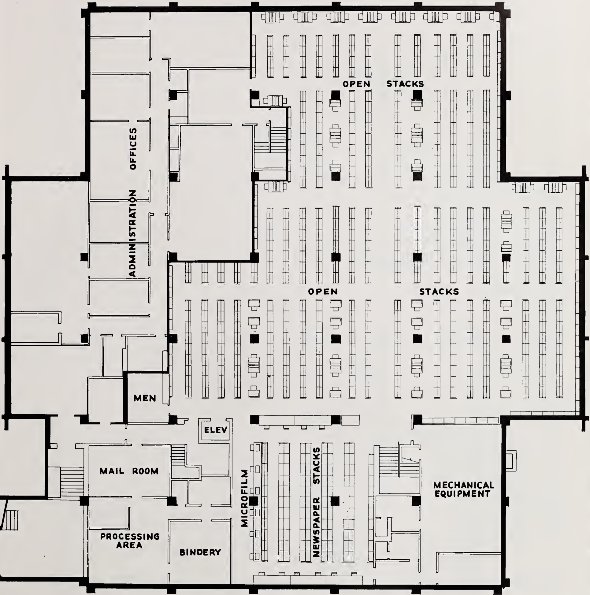
A-LEVEL PLAN
