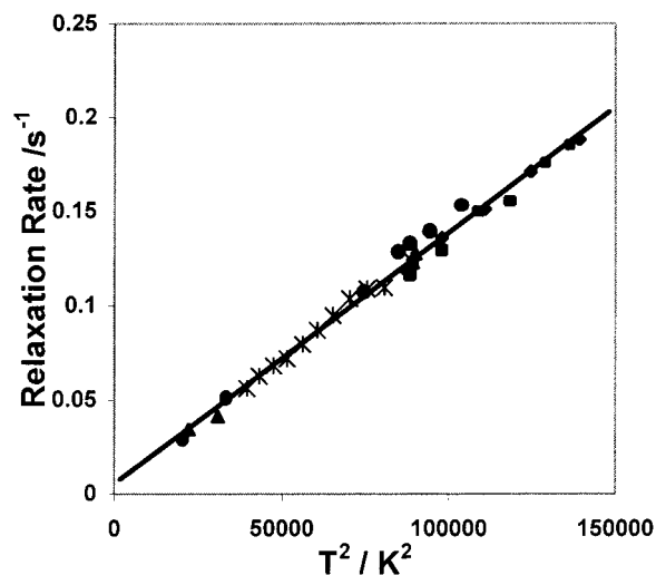
Figure 2. Best fit correlation of ^{207}\text{Pb} spin–lattice relaxation rate ( \text{s}^{-1} ) in solid \text{Pb}(\text{NO}_3)_2 vs temperature squared ( \text{K}^2 ): R = (1.33 \times 10^{-6} \text{ s}^{-1} \text{ K}^{-2})T^2 + 0.0056 \text{ s}^{-1} . Symbols are defined in Figure 1.
