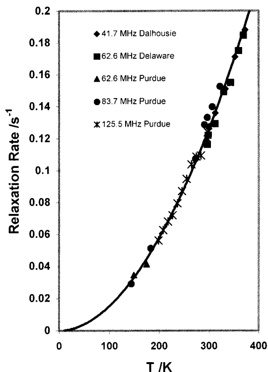
Figure 1. ^{207}\text{Pb} spin–lattice relaxation rate ( R/\text{s}^{-1} ) vs temperature ( T/\text{K} ) in solid \text{Pb}(\text{NO}_3)_2 at various field strengths. The best fit line is to the function R = (2.22 \times 10^{-6} \text{ s}^{-1} \text{ K}^{-1.92})T^{1.92} .
