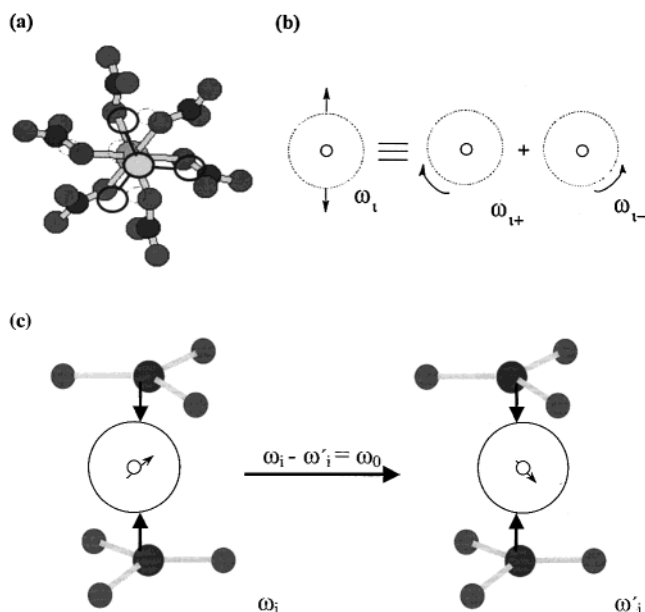
Figure 3. (a) Neutron diffraction structure of lead nitrate 20 viewed along [111] crystal axis. The uncoordinated axial nitrates are shown transparently. (b) The equivalence of a linear oscillator and a pair of counter-rotating oscillators. (c) Two low-frequency A_g phonons of the axial nitrates impacting the electron cloud (dotted) around the lead nucleus resulting in a nuclear spin flip.
