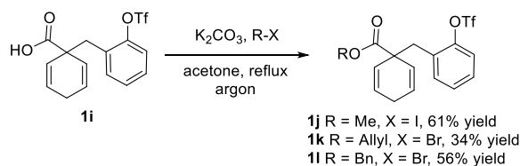
Scheme 2. Esterification reactions.
