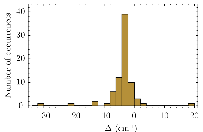
FIG. 9. Histogram of the discrepancy \Delta (current observations — previous calculations) from Table I. The average is -3.8 \text{ cm}^{-1} with a standard deviation of 5.3 \text{ cm}^{-1} .
