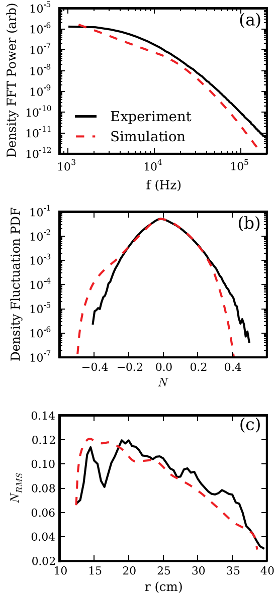
FIG. 2. (a) The power spectral density of the density fluctuations, showing the results from simulation versus experiment, (b) the probability distribution function of the density fluctuations, and (c) the RMS amplitude of the density fluctuations as a function of radius.
