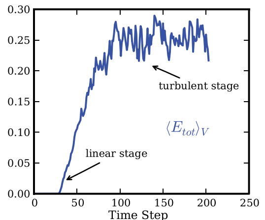
FIG. 3. Time evolution of the volume-averaged total energy. Each time step is 400/\omega_{ci} \sim 170 \mu s .
