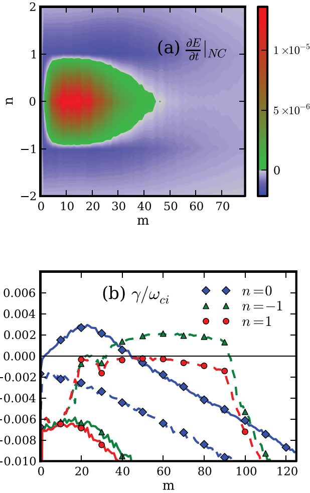
FIG. 8. (a) The total spectral nonconservative energy injection \frac{\partial E(\vec{k})}{\partial t}|_{NC} and (b) the spectral nonconservative growth rate spectrum \gamma_T(\vec{k}) of the turbulence compared to the linear growth rate spectrum, \gamma_L(\vec{k}) . The solid lines represent \gamma_T(\vec{k}) which is calculated using Eq. (17) averaged over the saturated turbulent phase, while the dashed lines represent \gamma_L(\vec{k}) and are calculated with the same equation using the linear phase of the simulation.
