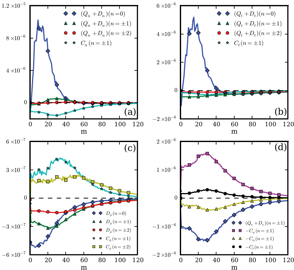
FIG. 6. (a) The solid curves quantify the energy dynamics of the density potential energy averaged over time during the saturated turbulent phase. The notation n \pm 1 represents the summation over the n = 1 and n = -1 curves. (b) The energy dynamics of the temperature potential energy, (c) the perpendicular kinetic energy, and (d) the parallel dynamics (adiabatic response). The contributions to C_t(\vec{k}) in (d) are broken up with C_t(\vec{k}) = -C_n(\vec{k}) - C_\phi(\vec{k}) - C_i(\vec{k}) . The density and temperature sources are neglected in (a) and (b), respectively. They only contribute at m=0 .
