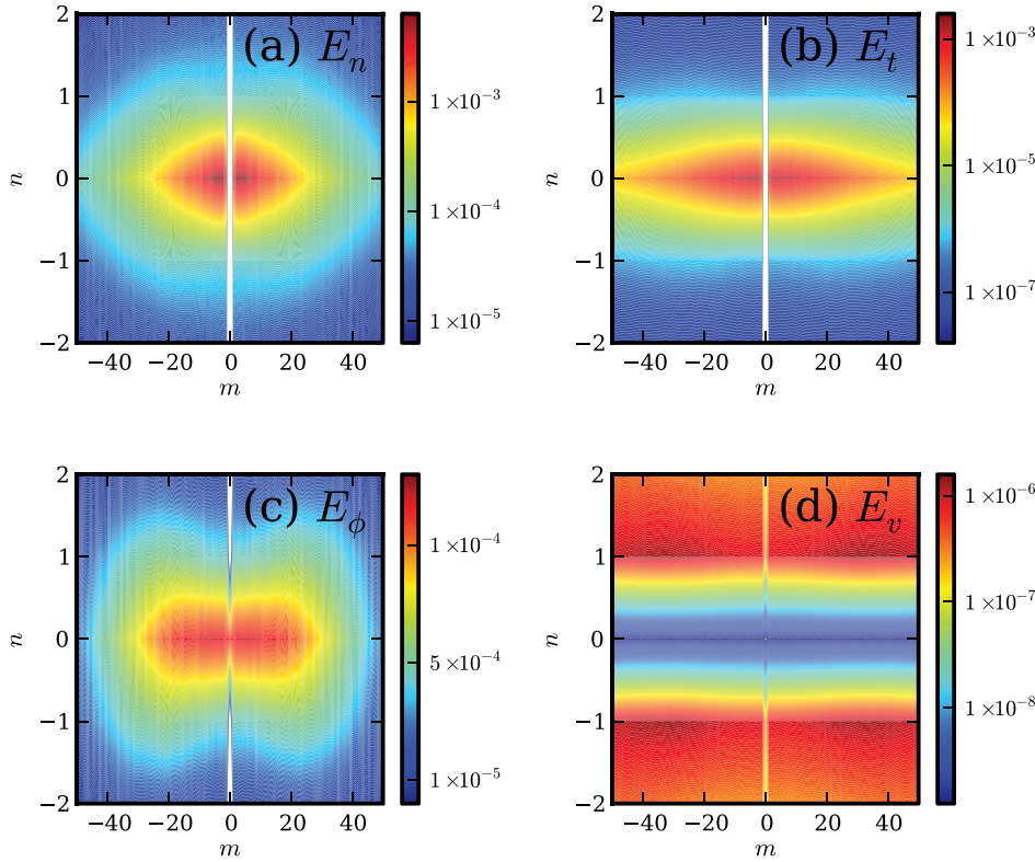
FIG. 4. (a) E_n(\vec{k}) , (b) E_t(\vec{k}) , (c) E_\phi(\vec{k}) , and (d) E_v(\vec{k}) in the m - n plane averaged over time during the saturated turbulent phase. Note the different scales used on each figure and also that the vertical white lines at m = 0 in (a) and (b) are due to the density and temperature sources which subtract out this component of the fluctuations. The zonal flow, defined as the n = 0, m = 0 component of the E \times B velocity, has an energy of magnitude of 1.4 \times 10^{-4} as seen in (c).
