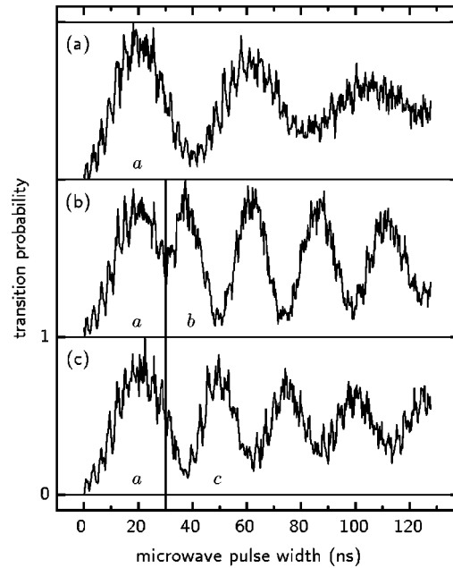
FIG. 9. Curve (a) shows the Rabi oscillations for a modulation amplitude at the highlighted point labeled a in the previous figure. In (b) and (c) there is a vertical line showing the time at which the rf amplitude was suddenly switched during the time scan to the value labeled b and c , respectively, in the previous figure.
