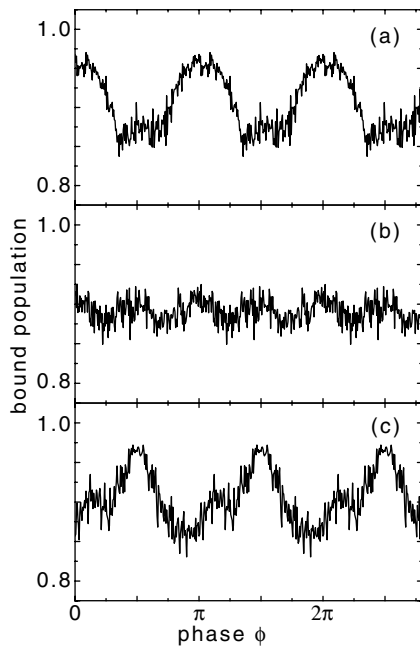
FIG. 4. One-dimensional model calculations for phase dependent ionization of wave packets near (a) \bar{n} = 75 , (b) \bar{n} = 67 , and (c) \bar{n} = 61 . The average ionization level is set to 10%.
