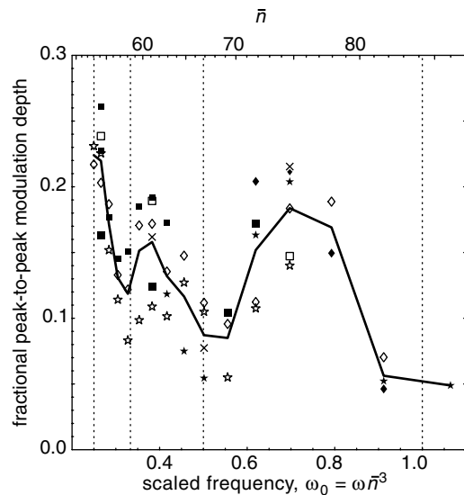
FIG. 2. Peak-to-peak modulation depth of the phase dependent ionization signals plotted versus scaled frequency. Different symbols represent data taken on different days and the solid line is the average of all data sets taken at a given laser tuning.
