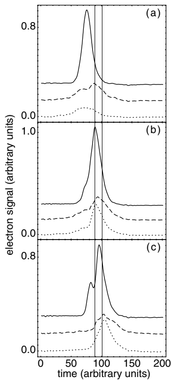
FIG. 3. State distributions for wave packets initially excited near (a) \bar{n} = 75 , (b) \bar{n} = 67 , and (c) \bar{n} = 61 . The solid curve is the state distribution for the initially excited wave packet. The dashed (dotted) curve is for ionization at phases of \phi = 0 and \pi/2 , indicated by the dashed (dotted) lines in Fig. 1. The vertical lines indicate the locations of \omega_0 = 1/2 (left) and \omega_0 = 1/3 (right).
