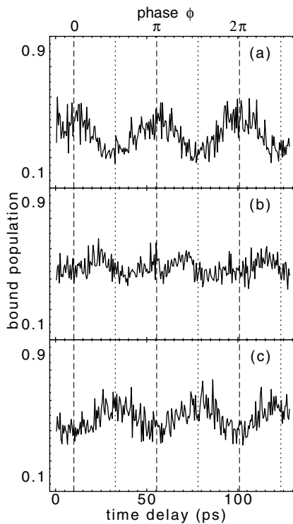
FIG. 1. Normalized remaining atom signals as a function of time delay of the mode-locked laser pulse for (a) \bar{n} = 75 , (b) \bar{n} = 67 , and (c) \bar{n} = 61 .
