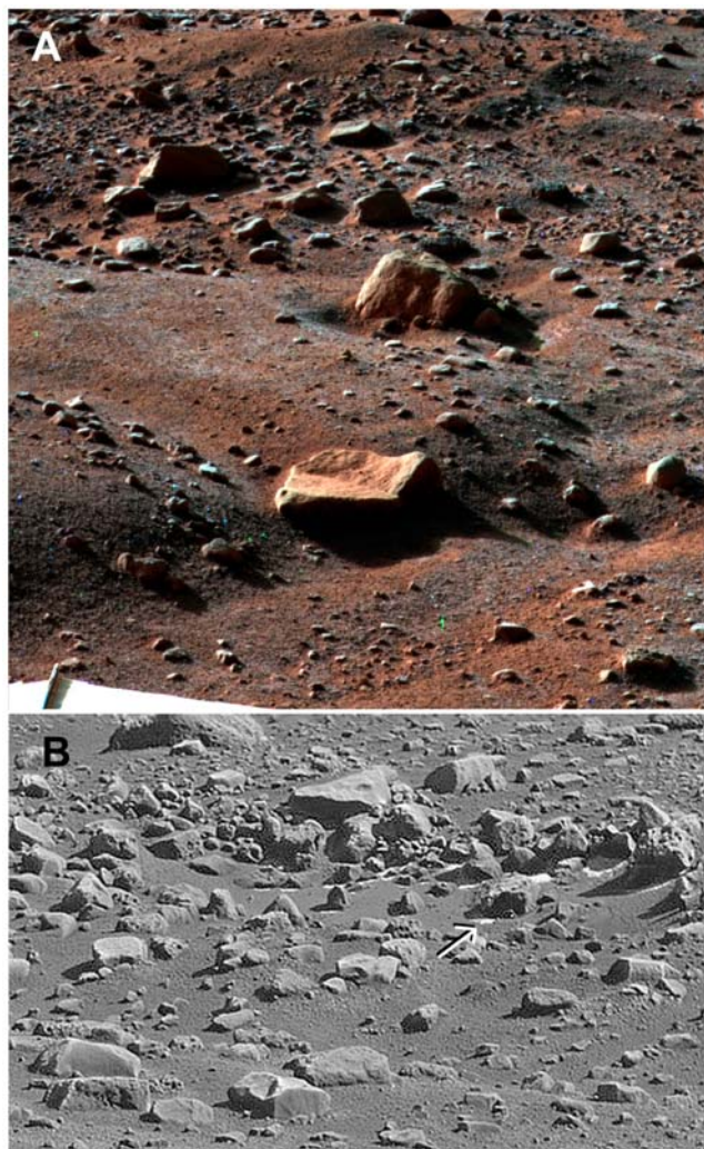
Figure 17. (a) SSI false color (R, 0.75 \mu\text{m} ; G, 0.53 \mu\text{m} ; B, 0.44 \mu\text{m} ) composite of “Winkies” (an \sim 27 cm rock in the foreground) on sol 79 at \sim 0600 LTST. White-blue frost is visible on the soil behind Winkies. (b) Ratio of SSI filters L2 to LC ( 0.445 \mu\text{m} to 0.967 \mu\text{m} ) for “Jumping Cow” area on sol 80 at \sim 1300 LTST. The white patches on the shadowed sides of the rocks are interpreted to be water ice.
