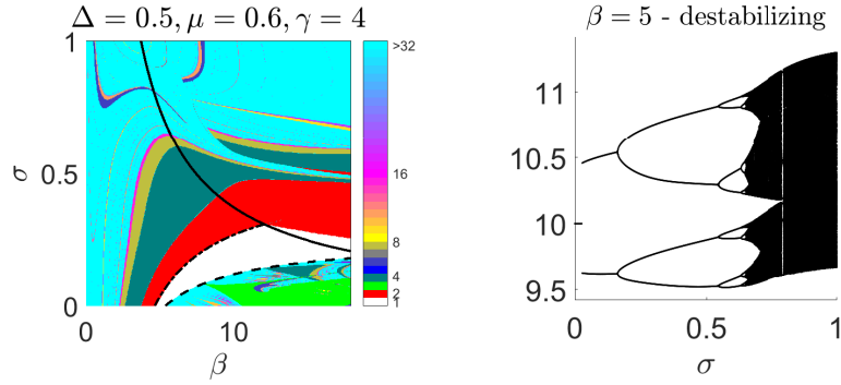
Figure 6: Two-dimensional bifurcation diagram (left plot). The solid, dashed and dash-dotted curves represent the bifurcation curves (iv'), (i') and (ii') in (30) in the Appendix, respectively. The right plot represents the evolution of the stock price on varying \sigma .
