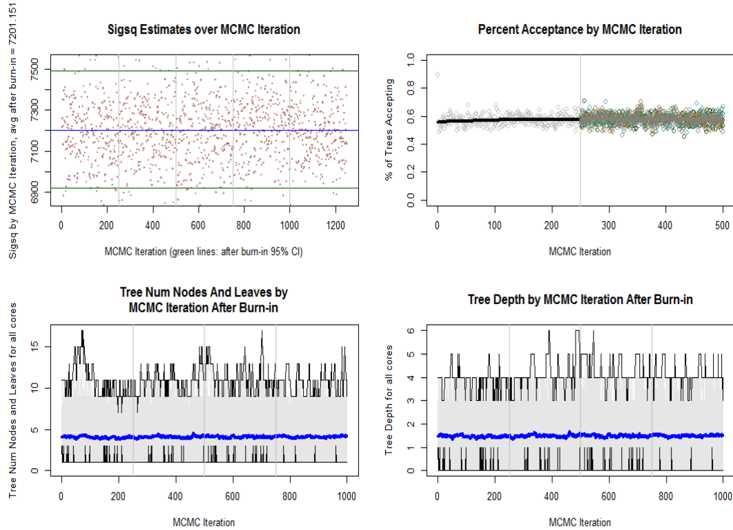
Figure 7: Convergence diagnostic
