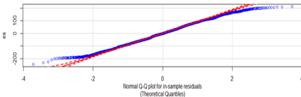
Figure 6: Assessment of Normality
