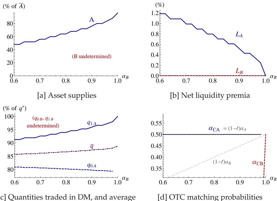
Figure 9: Comparative statics with respect to \alpha_B , with a little bit more IRS ( \rho = 0.02 ).
