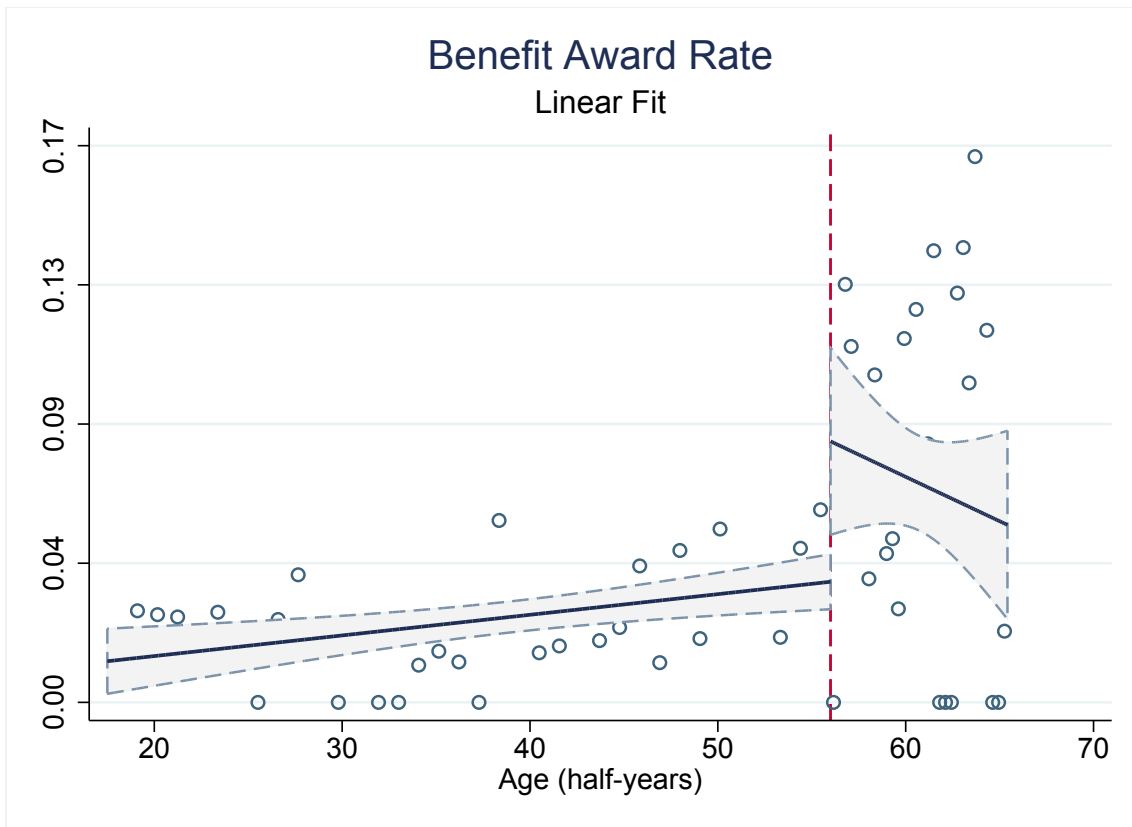
Figure 2: Discontinuity in the Benefit Award Rate
