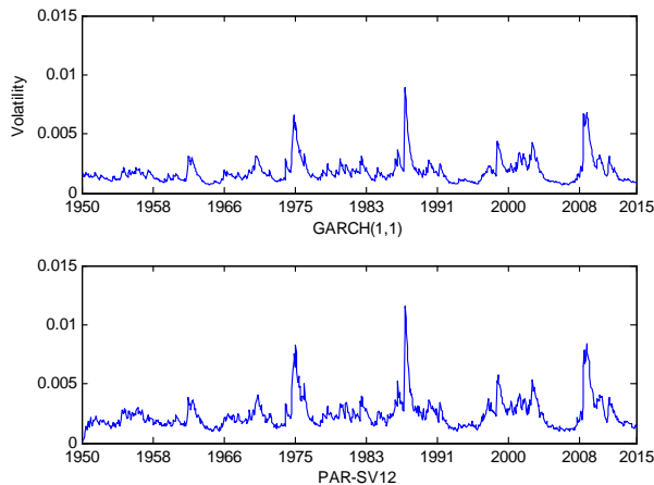
Figure 5.11: Volatilities induced by the GARCH(1,1) and PAR-SV_{12} .
