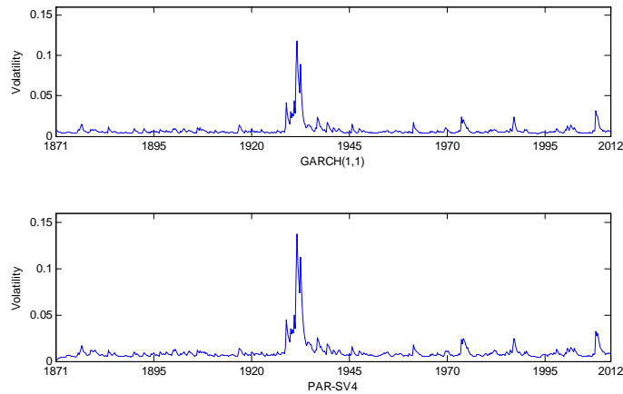
Figure 5.8: Volatilities induced by the GARCH(1,1) and PAR-SV_4 .
