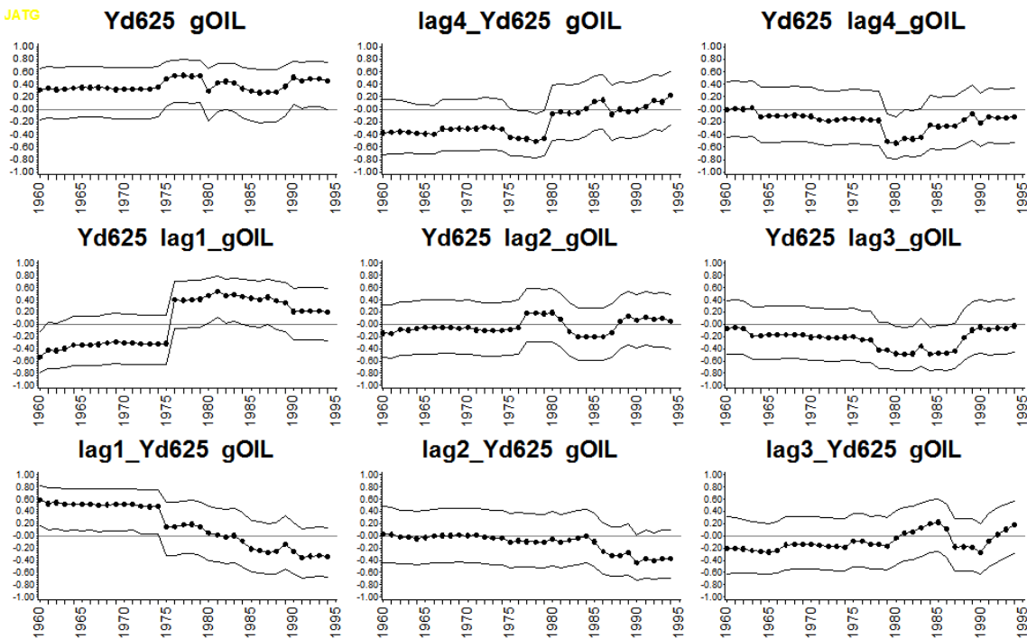
Figure A2. Correlations between gOIL and Yd625 at lags 0 to 4. All specifications as in Figure A1 but with 20-year rather than 30-year samples.
