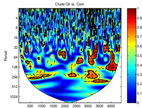
Chart 6: Continuous Wavelet Transform – Gold vs. Crude Oil Chart 7: Continuous Wavelet Transform – Crude Oil vs. Corn
