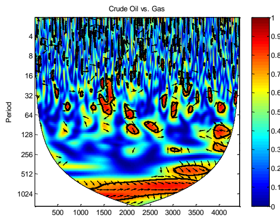
Chart 9: CWT – Crude Oil vs. Gas
