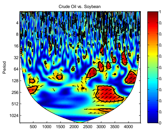
Chart 8: CWT – Crude Oil vs. Soybean
