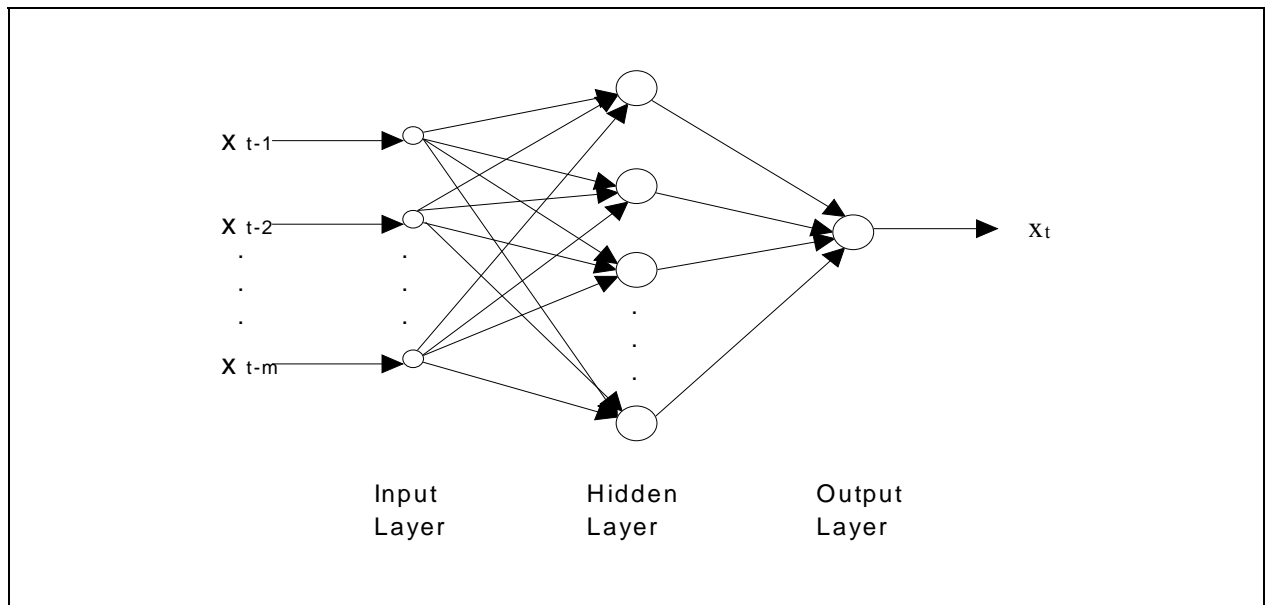
Figure 1 : The m-d-1 neural network architecture
