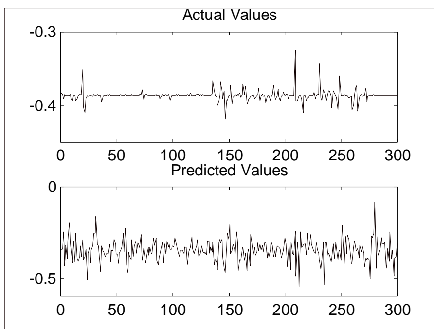
Figure 17: FF/GRD actual and predicted interest rates series using a RBF neural network with genetic algorithms.
