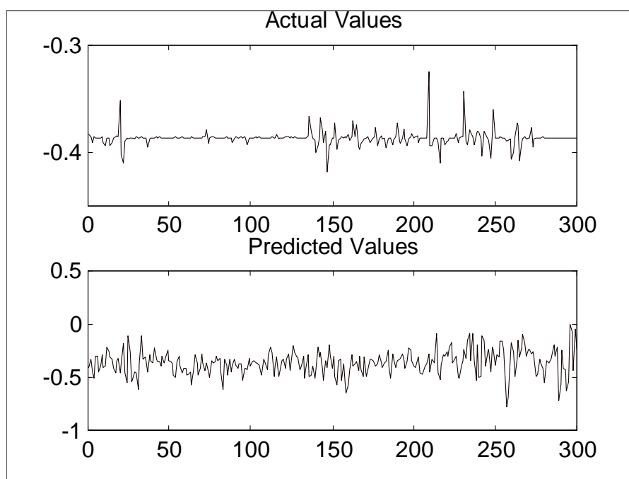
Figure 18: BP/GRD actual and predicted interest rates series using a RBF neural network with genetic algorithms.
