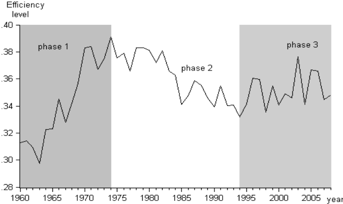
Figure 4: Efficiency of the Greek energy system
