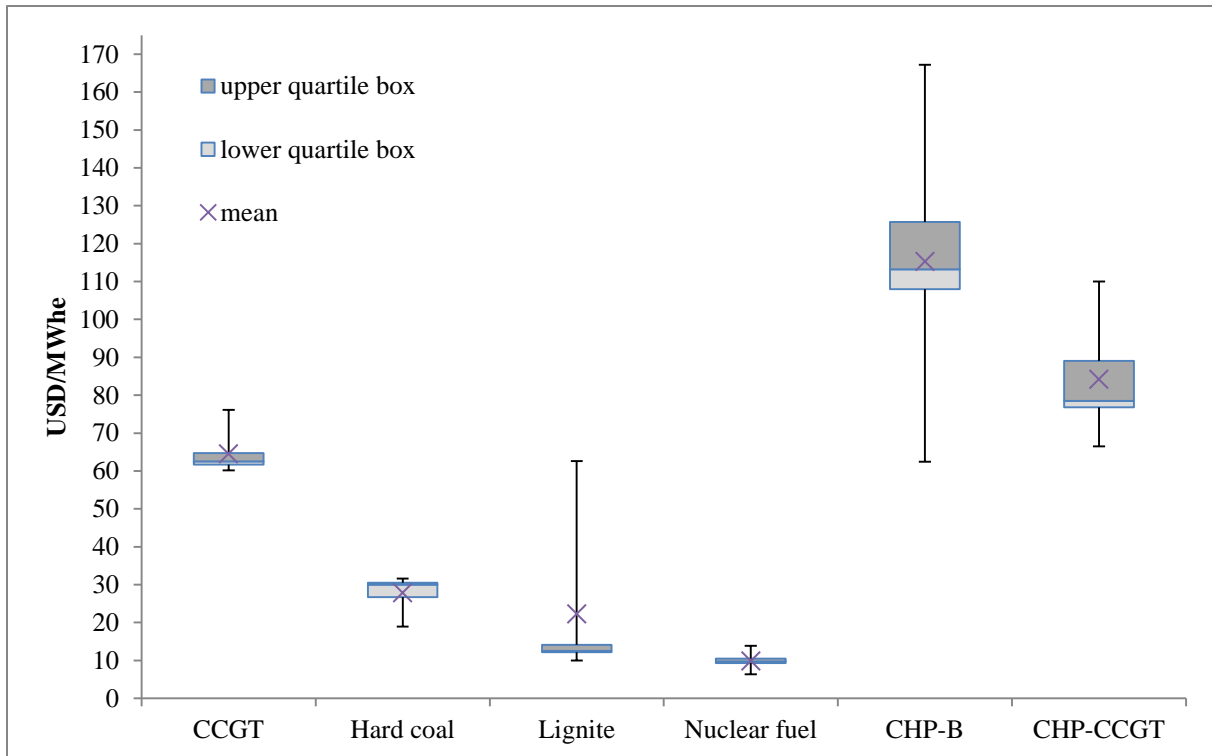
Figure 8. Levelised fuel costs presented in the reviewed studies (i.e. [4], [5], [7], [8], [10], [12], and [14]) . The cost figures are visualized in box plots showing the minimum value, lower quartile, median, upper quartile, and the highest value. The mean value is also included in the figure. Note that CHP-W fuel costs are omitted, since the costs tend to be negative due to gate fees. Reported fuel cost figures for CHP-W is in the range between -98 USD/MWhe and -246 USD/MWhe.
