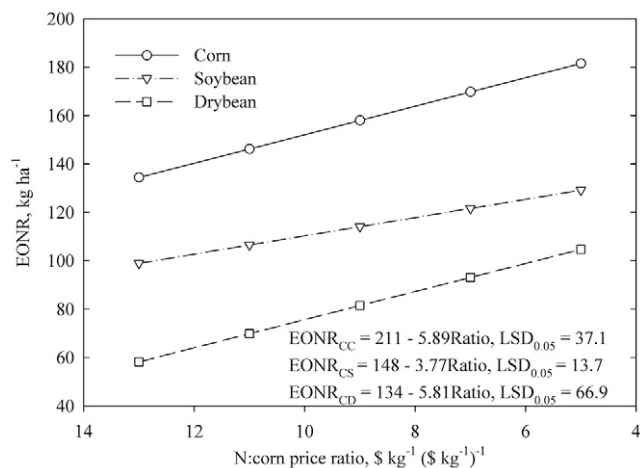
Fig. 3. The effect of the N/corn price ratio on the economically optimal nitrogen rate (EONR) determined for corn following corn ( n = 12 , CC), soybean ( n = 16 , CS), and drybean ( n = 4 , CD) in rotation as determined from 32 irrigated trials conducted in Nebraska in 2002–2004.
