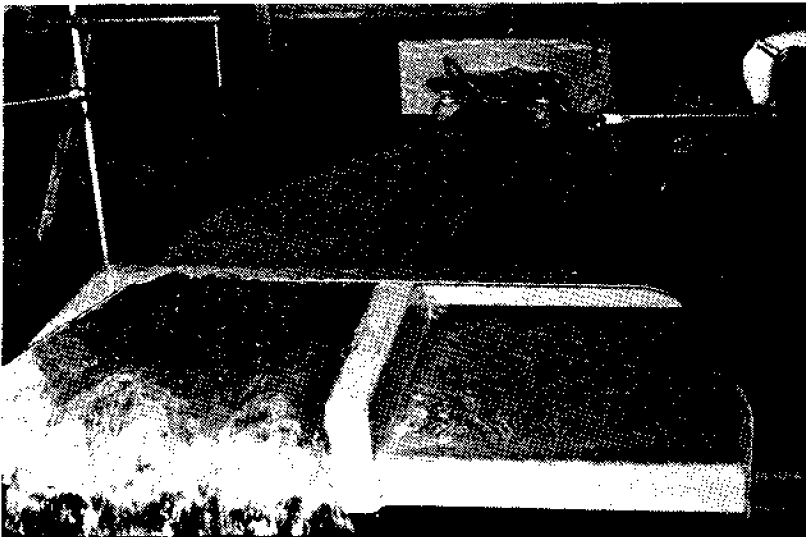
Figure 10. Five-inch fiber glass fluidic diverter. The total discharge, 2.5 cfs, is switched from one outlet to the other by the diaphragm valve on the air vent at the contracted section.
