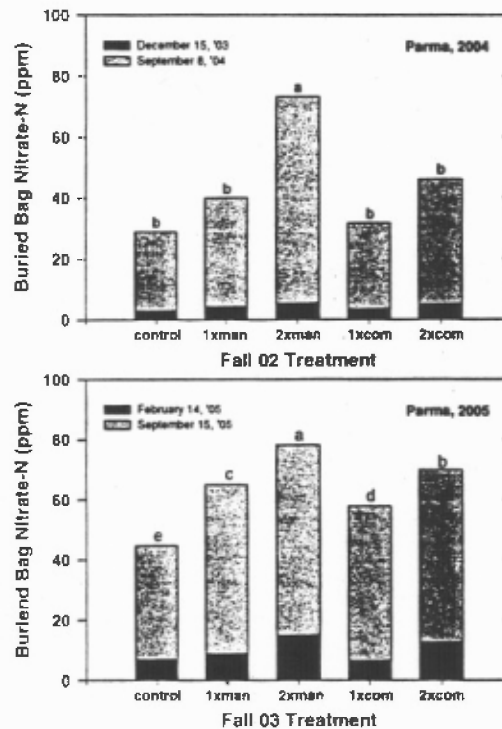
Figure 9. Buried bag \text{NO}_3\text{-N} following the planting of wheat as affected by organic N sources applied for the previous season sugarbeets.
