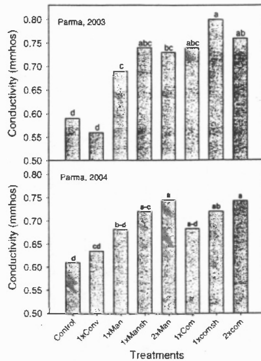
Figure 6. Sugarbeet brei conductivity in 2003 and 2004 as affected by treatments
