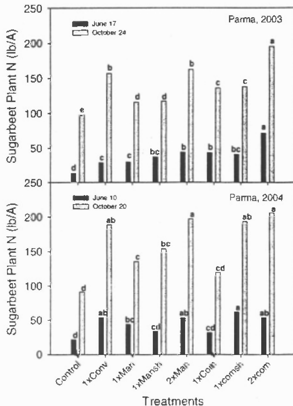
Figure 3. Early season and pre-harvest sugarbeet N uptake in leaves and roots.
