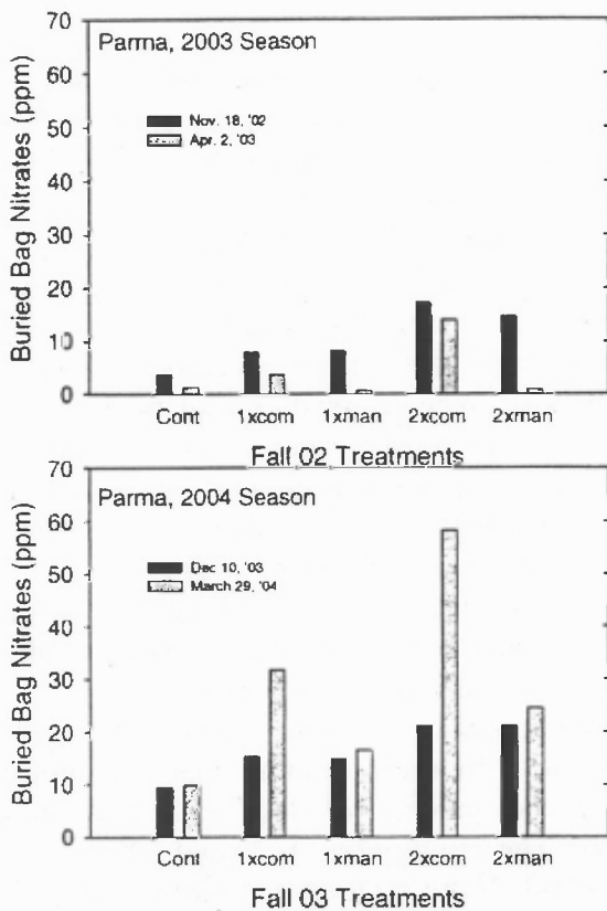
Figure 1. Over-winter N mineralization based on buried bag \text{NO}_3\text{-N} in the fall after organic N was incorporated and in early spring prior to sugarbeet planting.
