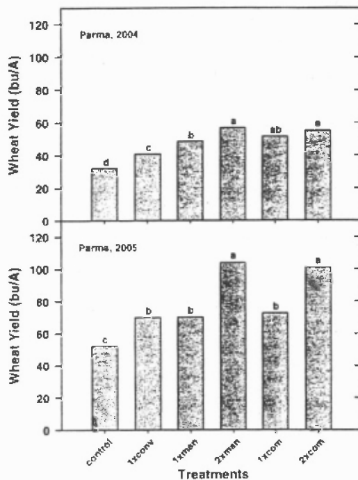
Figure 8. Grain yield in 2004 and 2005 as affected by treatments applied for sugarbeets the previous season
