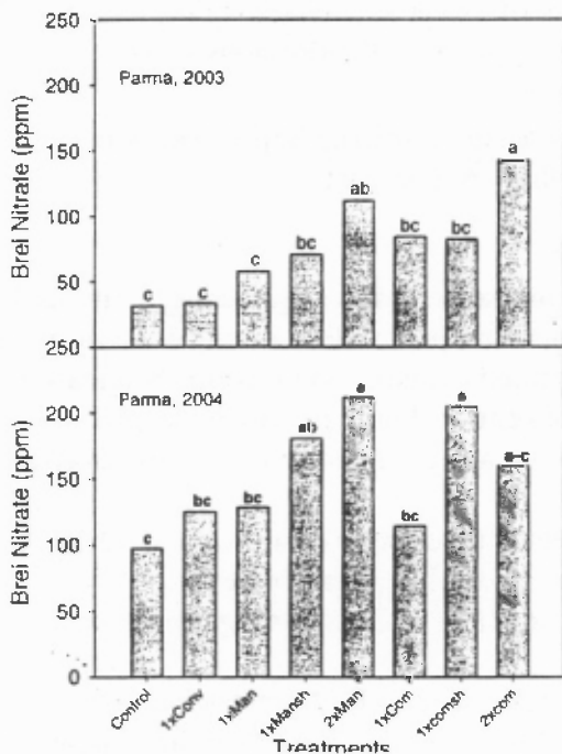
Figure 7. Sugarbeet brei nitrate in 2003 and 2004 as affected by treatments.
