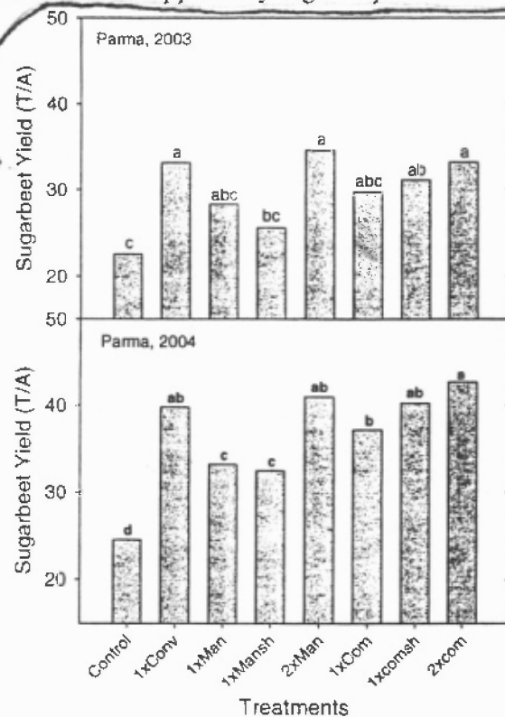
Figure 4. Sugarbeet yield in 2003 and 2004 as affected by N treatments.
