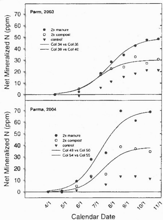
Figure 2. Net N mineralization as affected by untreated and 2x available N rates of manure and compost during the sugarbeet season.
