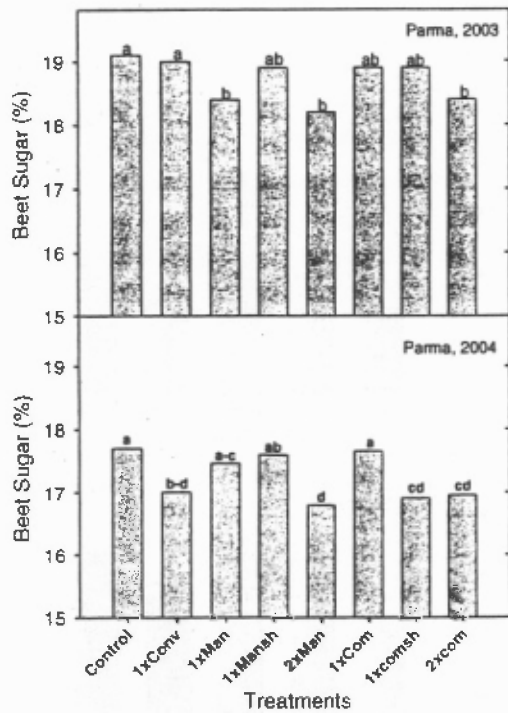
Figure 5. Sugarbeet percent sugar in 2003 and 2004 as affected by treatments.
