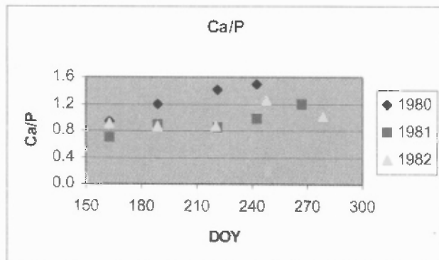
Figure 12. The ratio of Ca/P (mg/kg) in blood serum of cattle grazing forage on revegetated rangeland in the Shirley Basin of southeastern Wyoming.
