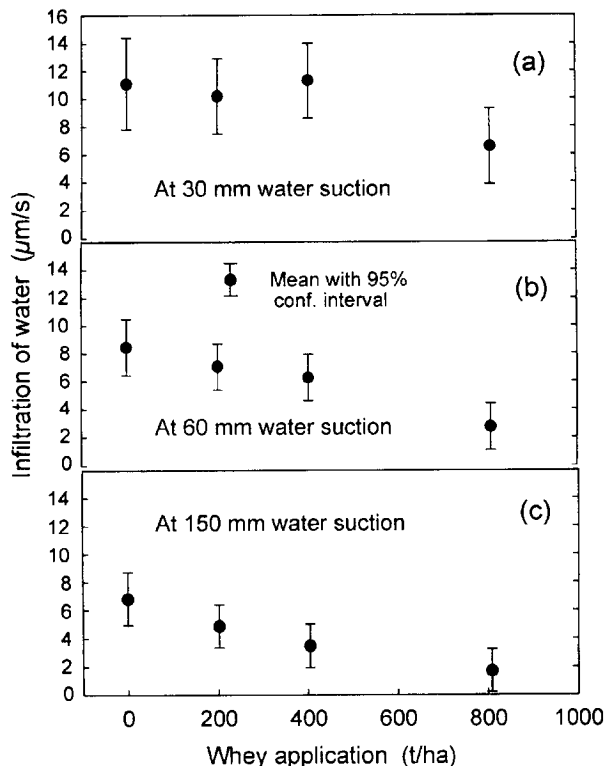
Fig. 1. Whey effects on the infiltration rate of water at suctions of 30, 60, and 150 mm of water.
