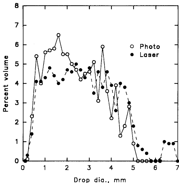
Figure 2—Drop size distributions by photo and laser methods for an impact sprinkler at 206 kPa pressure and 3.7 mm nozzle (Test 5).
