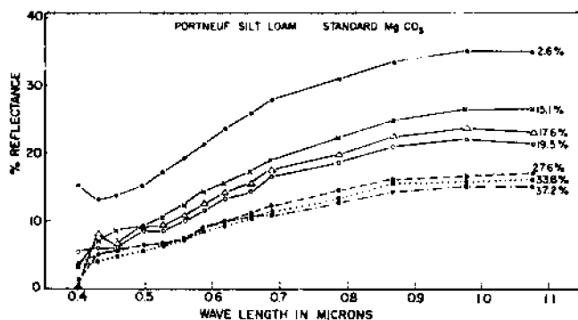
Fig. 4. Reflectance curves from Portneuf silt loam. Each curve represents a different percent moisture on a weight basis.
