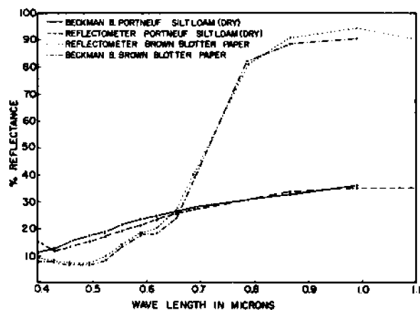
Fig. 6. Comparison of reflectance spectra secured with a Model B Beckman Spectrophotometer and the fabricated portable reflectometer.
