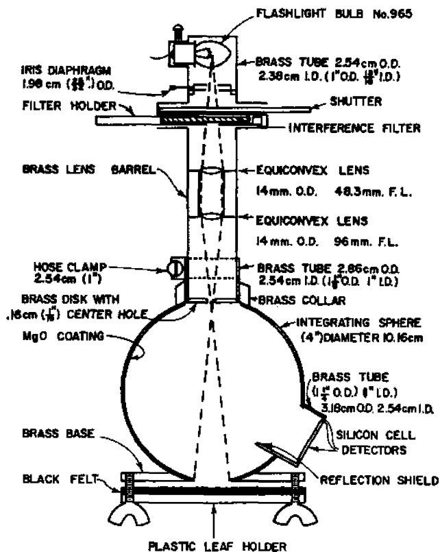
Fig. 1. Portable reflectometer for reflectance measurements from soils and plant leaves.
