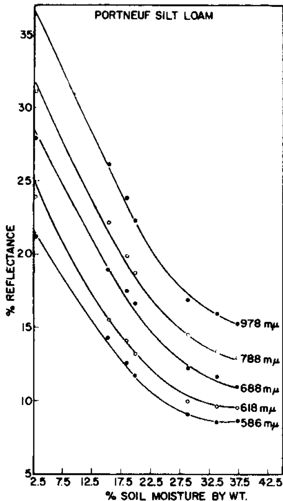
Fig. 5. Reflectance versus soil moisture at particular wavelengths.
