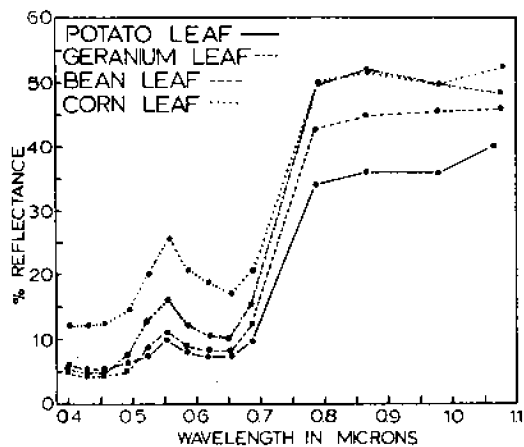
Fig. 3. Reflectance spectra from intact plant leaves.
