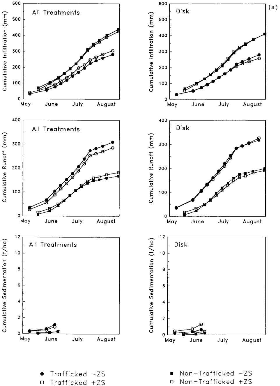
Fig. 1. Seasonal cumulative infiltration, runoff, and sedimentation patterns for 1989; (a) mean fall tillage and fall disk responses; (b) fall chisel and fall plow responses. Use or non-use of zone subsoiling is indicated by +ZS or -ZS, respectively.
