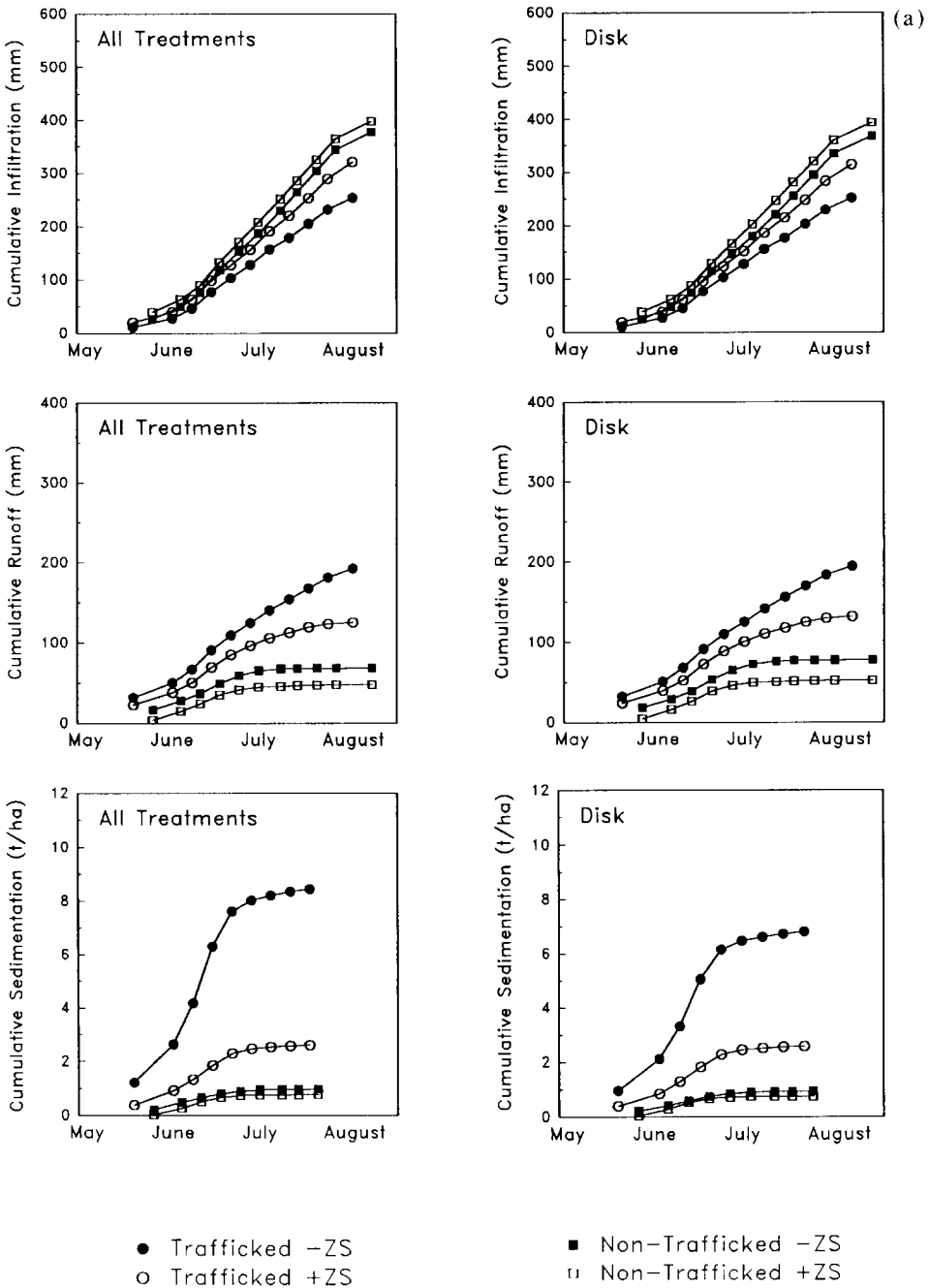
Fig. 2. Seasonal cumulative infiltration, runoff, and sedimentation patterns for 1990; (a) mean fall tillage and fall disk responses; (b) fall chisel and fall plow responses. Use or non-use of zone subsoiling is indicated by +ZS or -ZS, respectively.
