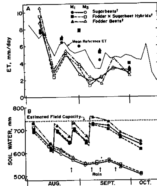
Figure 2. Measured soil water content and evapotranspiration, mean reference ET, and estimated field capacity for 1980 [Estimated field capacity determined at 0.33 bar. Mean (3-day) reference ET (alfaifa) determined by methods of Wright (23)]. + Sugarbeets = GWD2, AH10, LHY-1, and LHS-1; Fodder x Sugarbeet hybrids = Monorosa and Monoblanc; Fodder beets = Pajbjerg Korsroe and Rota.
