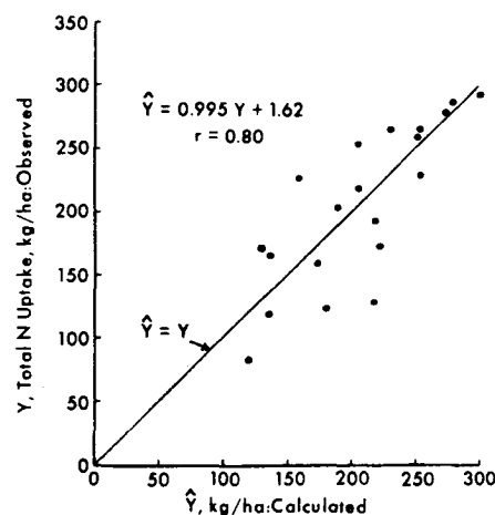
Fig. 4. Observed (Y) vs. calculated (Ŷ) N uptake by sugarbeets where Y = 0.75X_1 + 0.69X_2 + 1.3 (X 1 = residual NO 3 -N in root zone; X 2 = estimated N mineralized under prevailing temperature and water regimes).
