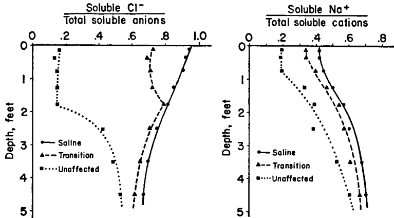
FIG. 2. Average ratios of soluble \text{Cl}^- to total soluble anions in relation to depth for soils of the three sampling categories.
