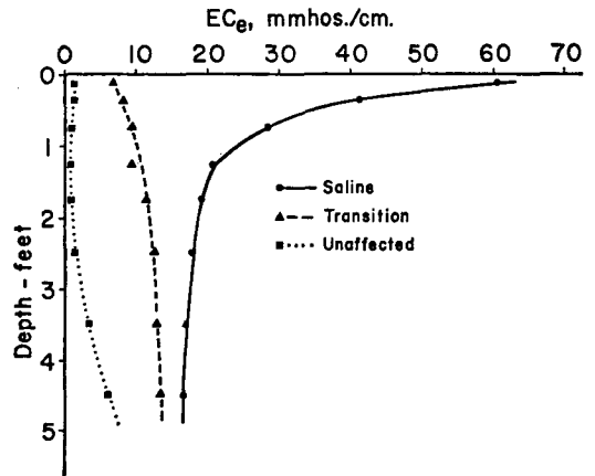
FIG. 1. Average salinity level in relation to depth for soils of the three sampling categories.
