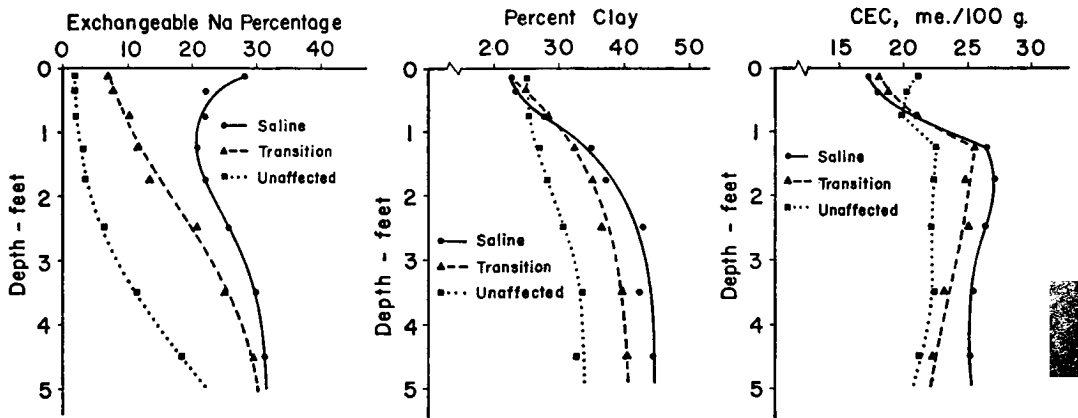
FIG. 4. Average exchangeable Na percentage in relation to depth for soils of the three sampling categories.
