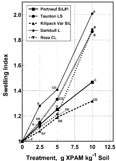
Fig. 5. Swelling index of XPAM-treated soils. The index was calculated as a ratio of soil column length at 1 h divided by the mean soil column length of the 0 g kg⁻¹ XPAM soil treatment. Symbols followed by the same letters indicate no significant difference between soil and XPAM treatments, determined from confidence limits constructed on treatment means ( P \leq 0.05 ).
