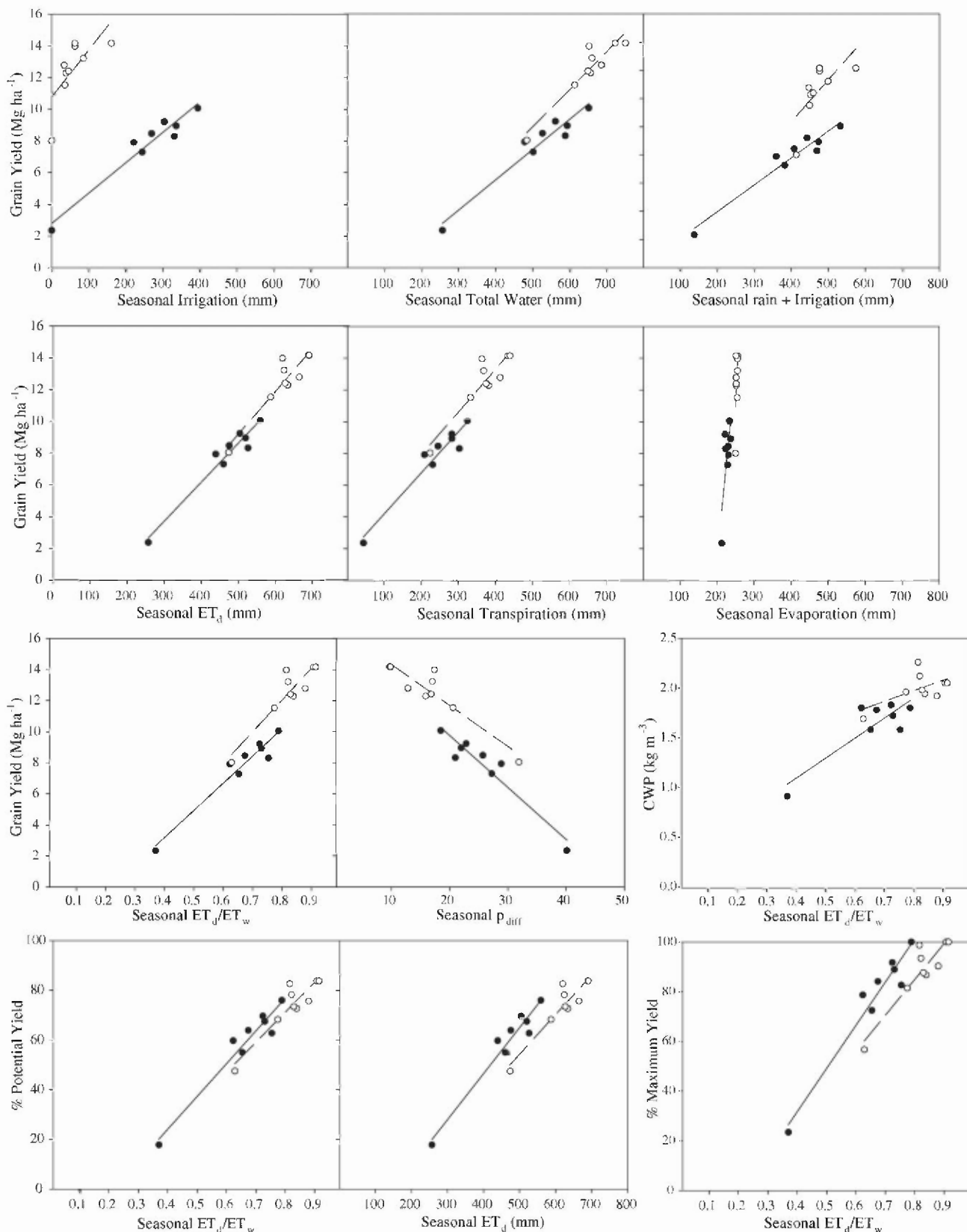
Fig. 3 – Relationships among different variables for corn obtained at North Platte during 2003 (solid circles) and 2004 (open circles). ET_d and T_d are actual crop evapotranspiration and transpiration, ET_w and T_w are crop evapotranspiration and transpiration when soil water is not limiting, p_{diff} is daily positive difference between the actual and the theoretical fraction of total available soil water in the root zone that can be depleted before moisture stress occurs, accumulated for the entire season, and CWP is crop water productivity. The solid and dashed lines are linear regression lines.
