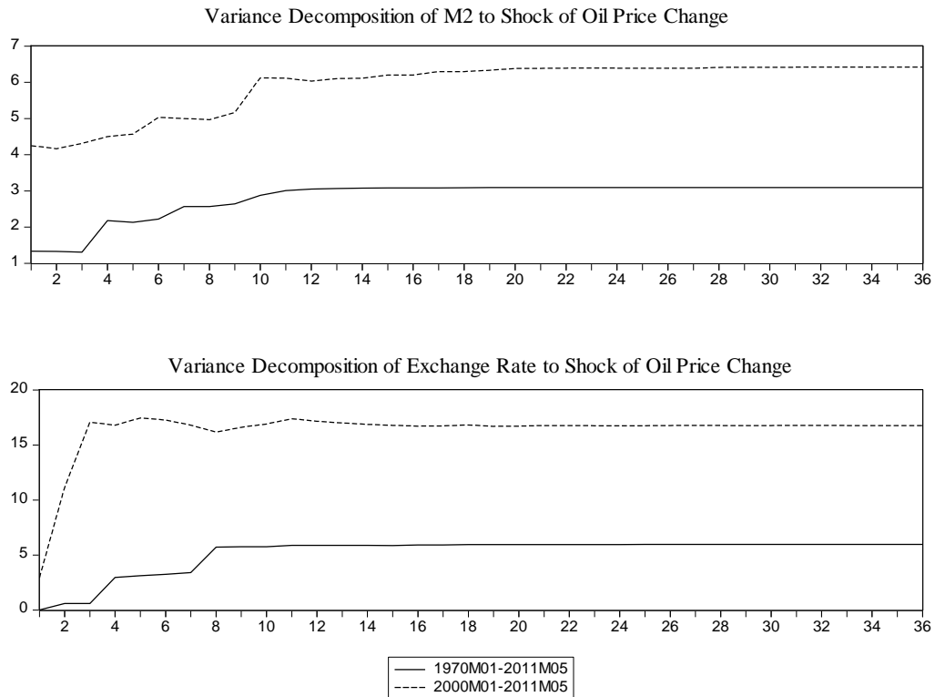
Figure 9. Variance Decompositions
