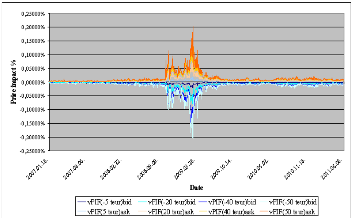
Figure 7: The time series of the virtual price impact function
