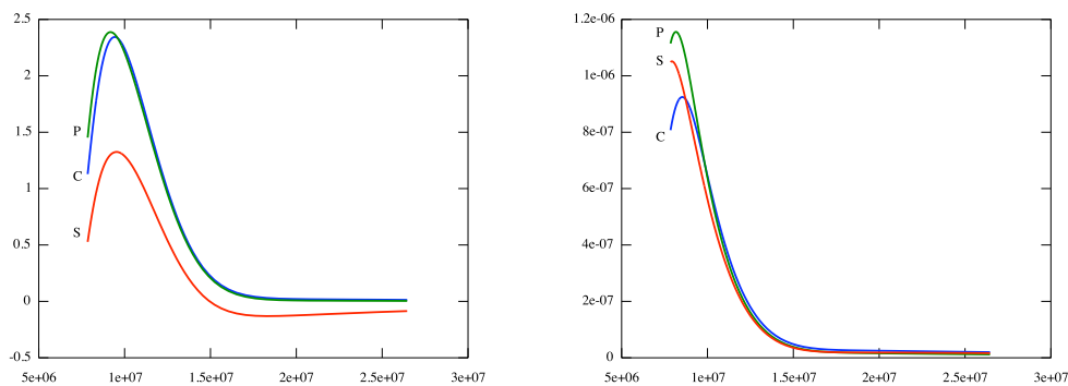
FIGURE 4. Sensitivity of distress exposure \hat{Q}_f (left) and distress pervasiveness \hat{b} (right) to an initial bankruptcy of size \hat{Q}_n , i.e. \partial/\partial\hat{Q}_n . Plot is for n = 10 counterparties each with capital K = \$1 million and positions equivalent to OTC contracts with \text{sd}(\text{exposure}) = \$1 million. Lines C , P , and S correspond to a market with a central counterparty, pooled OTC buyers and sellers, and separated buyers and sellers.
