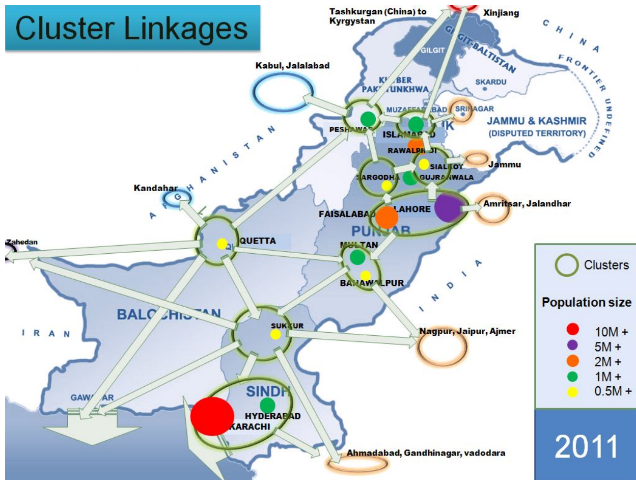
Figure 5: Cluster Linkages
