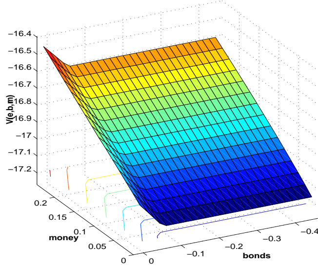
Figure 1: Value function as a function of m and b .
