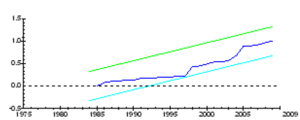
Fig 3.2: Cumulative Sum of Square Recursive Residual
