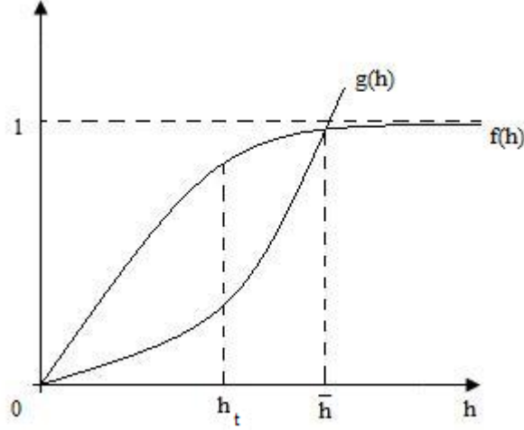
Figure 1: Unique steady-state equilibrium
