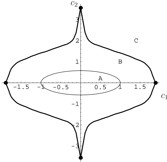
Figure 7. Strict and second-order stationarity regions of the model (25) with \epsilon_t \sim \mathcal{N}(0, 1) . A: second order stationarity, A \cup B : strict stationarity, B \cup C : non second-order stationarity, and C: non strict stationarity.
