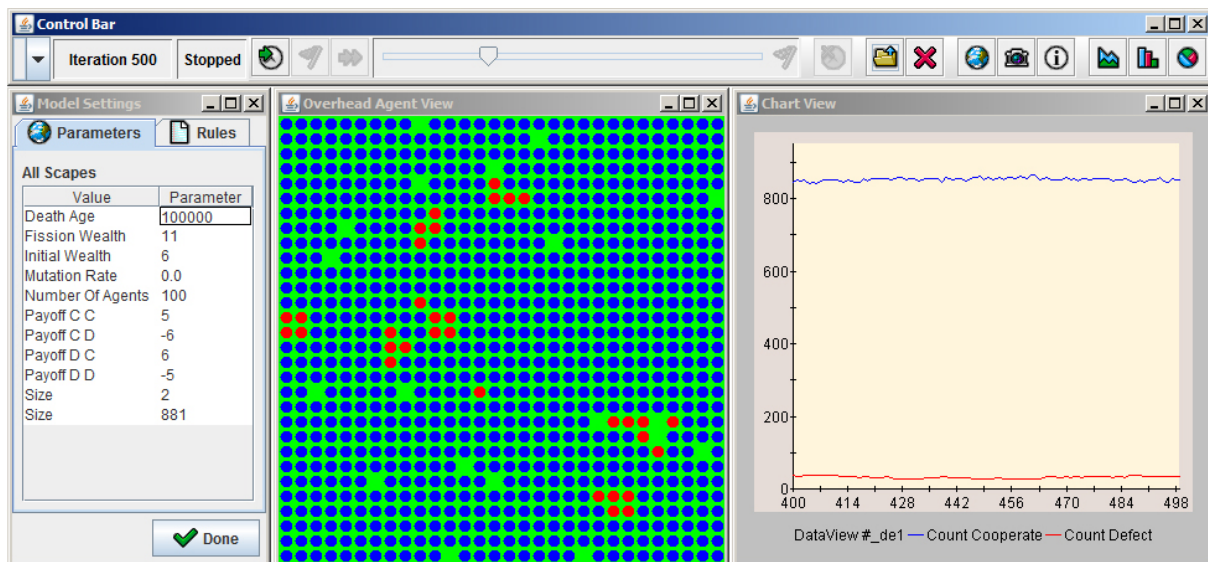
Image 1: Exemplary image of Run 1, re-implemented by Epstein in Ascape
