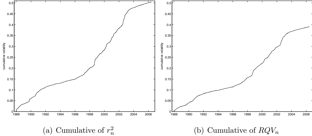
Figure 3: S&P 500 cumulative volatility over the years 1988–2006. Figure (a) estimates cumulative volatility by the sum of squared daily close-to-close returns. Figure (b) shows the cumulative of the daily realized variance, RQV_n , based on 81 five-minute returns.
