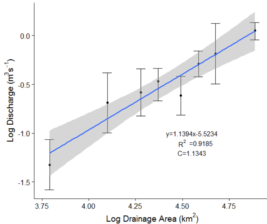
Figure 55. Peak discharge scaling relationship for Storm 21 (~ 1/17/17). Error bars represent upper and lower limit of the 95% confidence interval for that point's calculated discharge value.
