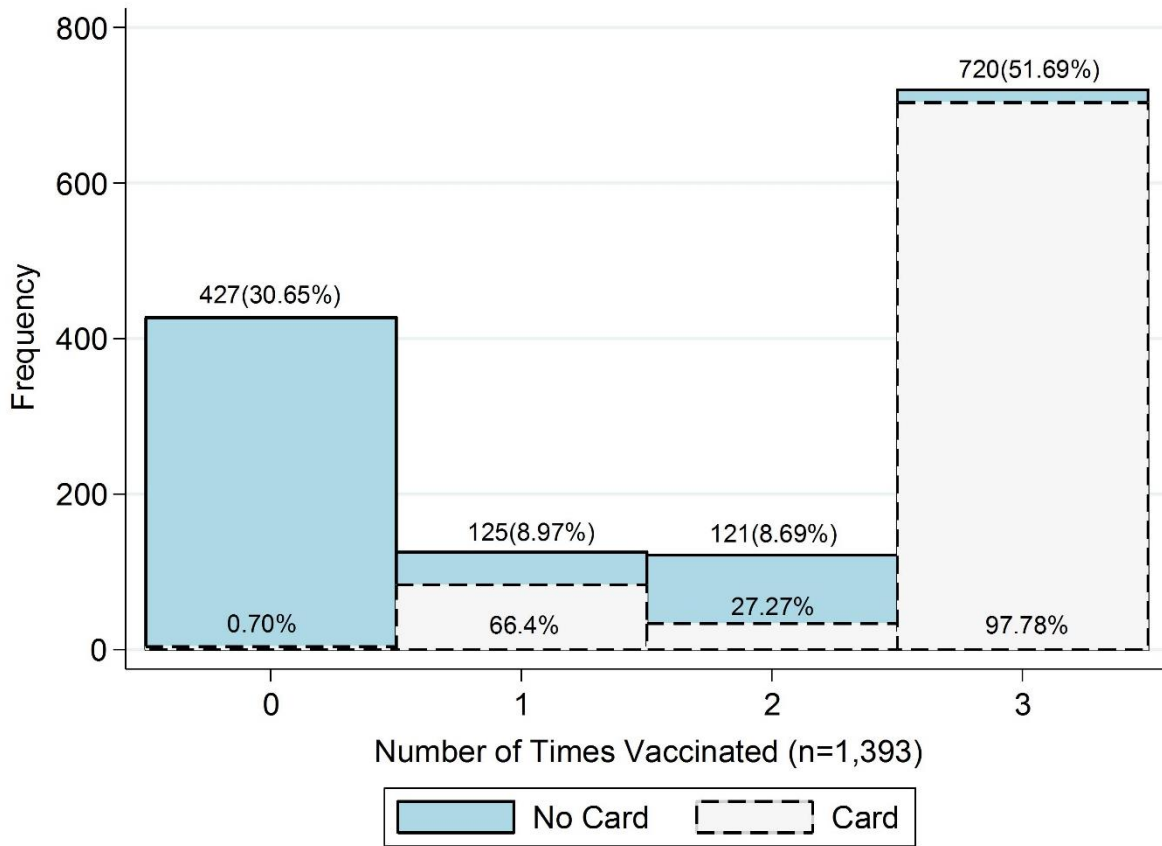
Figure 3 Histogram of the Number of Times Vaccinated by Immunization Card
