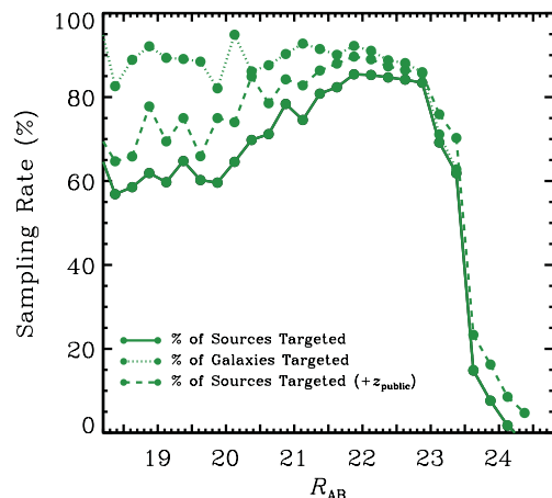
Figure 1. The ACES target sampling rate as a function of the R -band magnitude across the entire \sim 30 arcmin \times 30 arcmin COMBO-17/CDFS footprint. The target sampling rate is defined as the percentage of objects at a given R -band magnitude in the COMBO-17 photometric catalogue that were observed by ACES. The dotted and dashed lines show the sampling rate when only considering sources classified as non-stellar in the COMBO-17 catalogue (dotted) and when accounting for sources with a published spectroscopic redshift in the literature (dashed – see Section 2). To select the galaxy population, all sources classified as ‘Star’ or ‘WDwarf’ in the COMBO-17 photometric catalogue of Wolf et al. 2004 are excluded. At bright magnitudes, R_{AB} < 23 , ACES brings the target sampling rate in the CDFS to >80 per cent.
