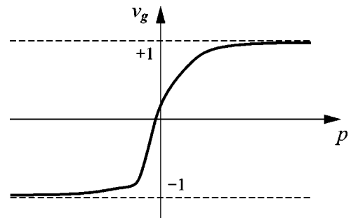
FIG. 8. Group velocity for the dispersion relation of the model in Fig. 7 as a function of the 3-momentum in a fixed direction. The modified dispersion has no group velocity exceeding 1. The dashed lines correspond to the usual limiting velocities \pm 1 .
