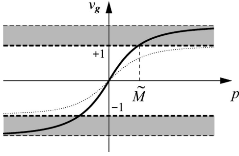
FIG. 4. Group velocity for the dispersion relation of the model in Fig. 3 as a function of the 3-momentum in a fixed direction. The asymptotic development of velocities exceeding 1 is apparent in the shaded region, which lies above a momentum scale \tilde{M} . The heavy dashed lines correspond to the usual limiting velocities \pm 1 . The dotted line is the usual result for a massive particle.
