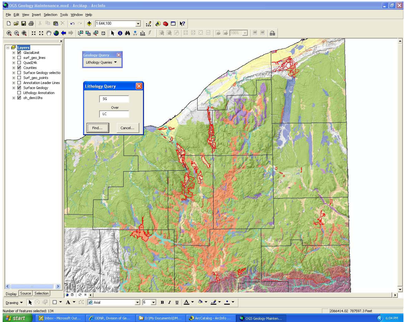
Figure 10. The Lithology Query toolbar with areas of sand and gravel (SG) overlying lake clay (LC) selected and outlined in red.
