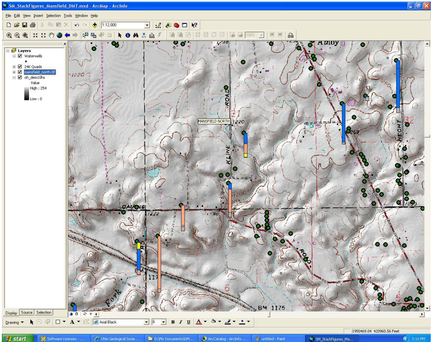
Figure 3. Selected water wells whose lithologic column is generated using the Stick-Figure Application . Colors in the stick figures represent various lithologies. Length of the stick figures corresponds to depth of the well, with deeper wells resulting in longer stick figures.
