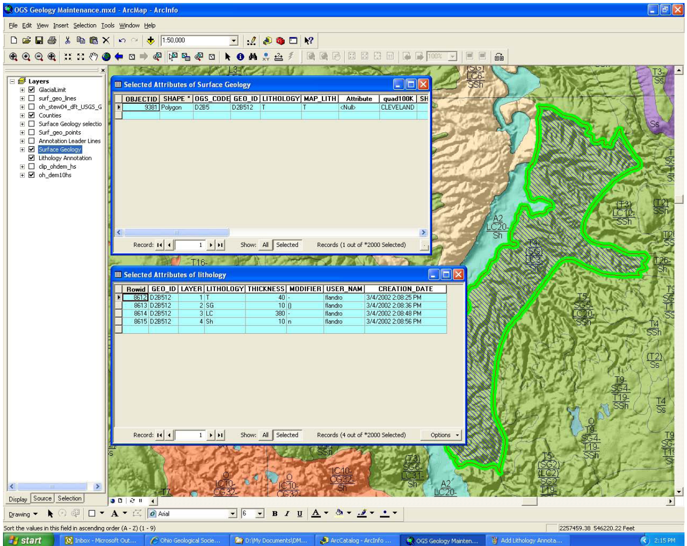
Figure 7. Example of the one-to-many relationship between the surface-geology polygon and the lithology table.
