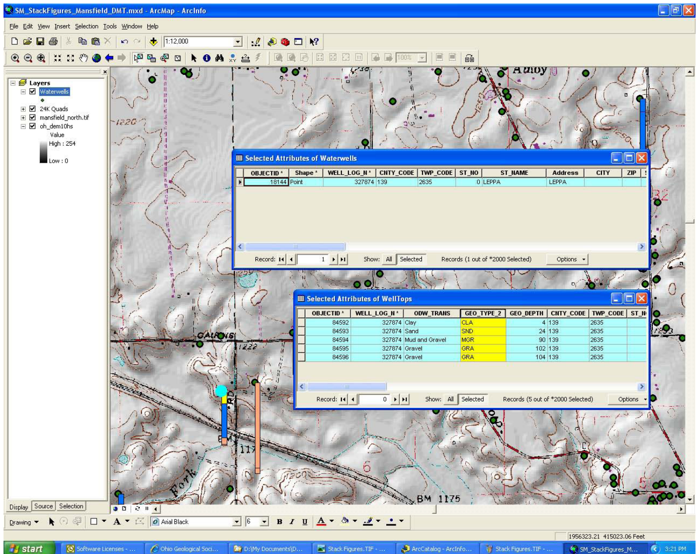
Figure 4. Example of the one-to-many relationship between the water-well location and the water-well log table. The well log record (upper table) is linked by WELL_LOG_N to the lithologies encountered downhole (lower table). The selected well is in the lower left-hand corner.
