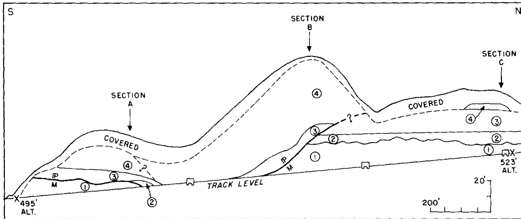
Figure 1.--Profile of west side of railroad cut at National Gypsum Co. plant near Shoals (Stop 3), Approximately to scale; vertical exaggeration 5 times.
