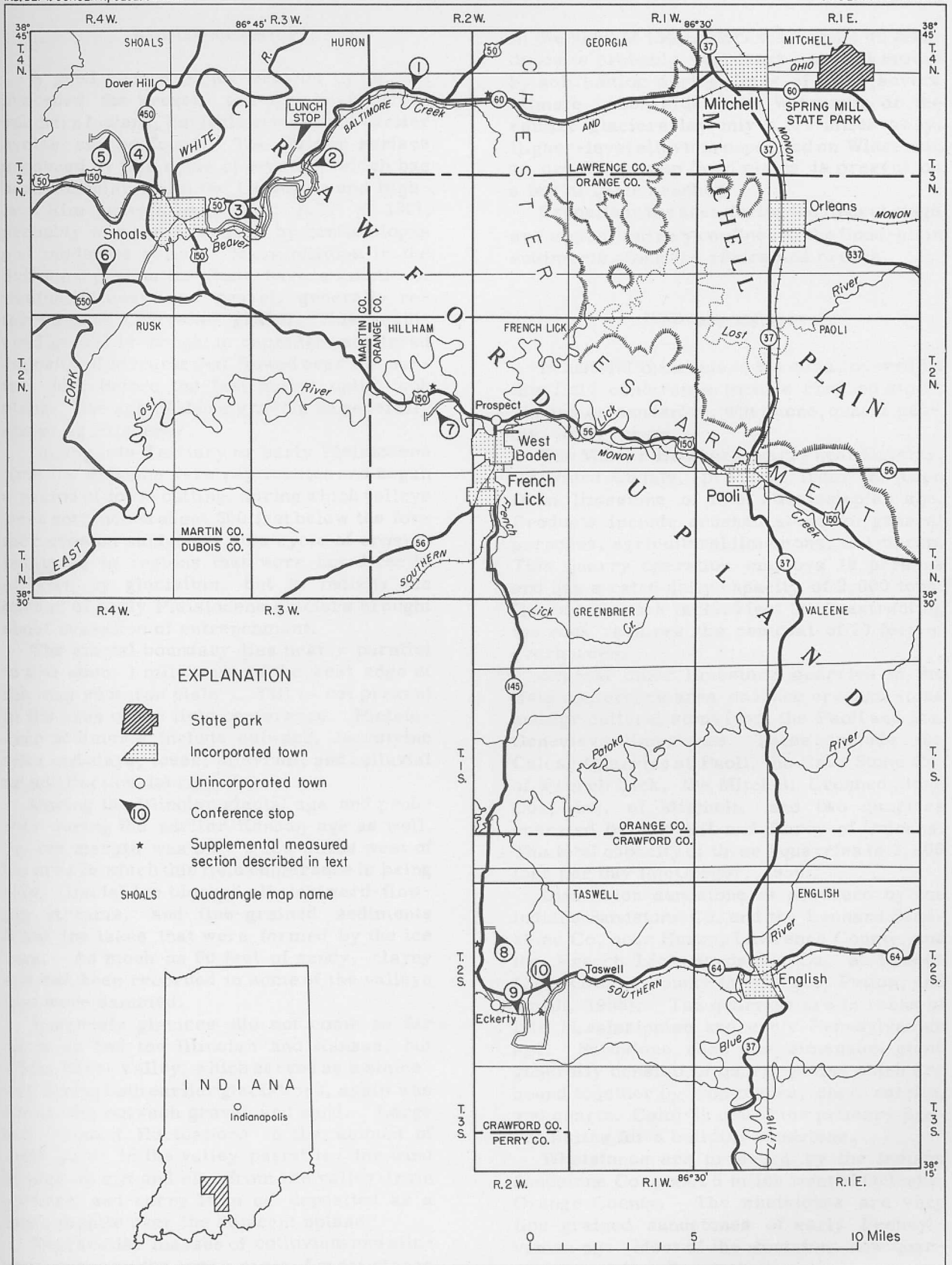
MAP OF FIELD CONFERENCE AREA SHOWING PHYSIOGRAPHIC UNITS
